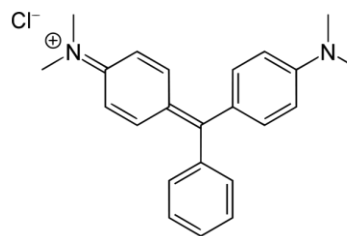
Figure 2 Chemical structure of malachite green
